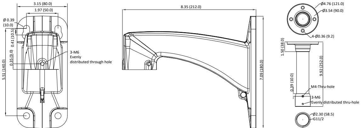
Wall Mount
